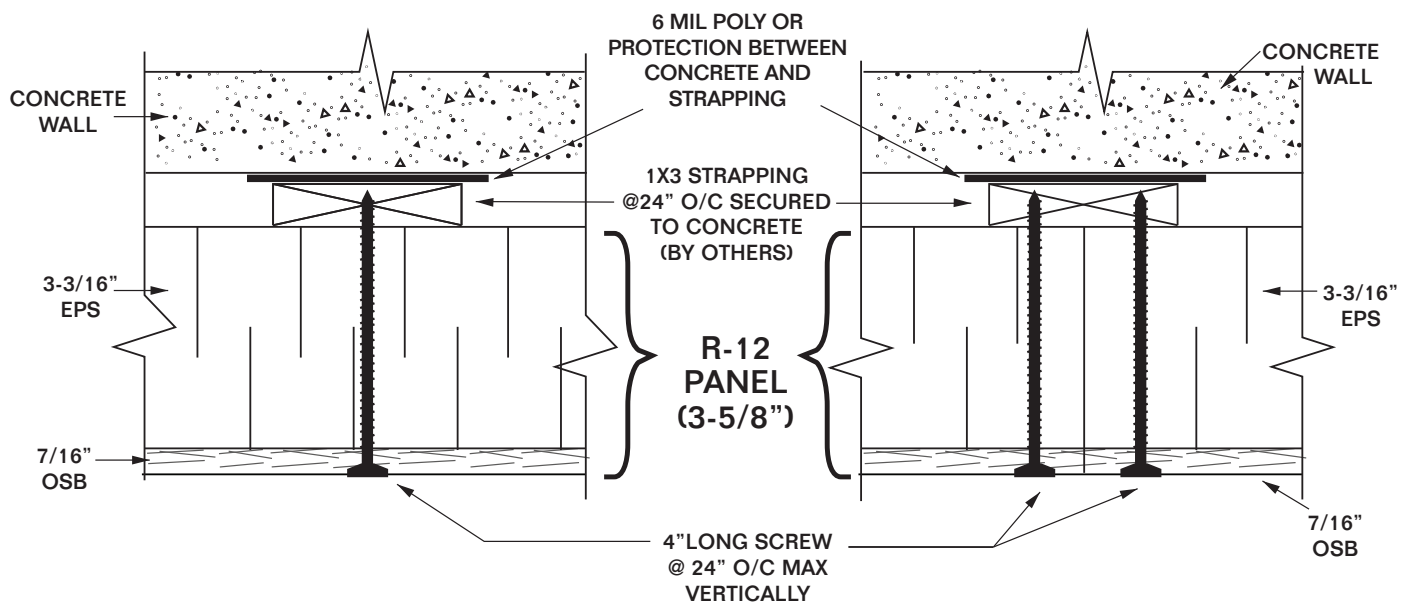
PLAN DETAIL "A" (AT PANEL INTERIOR)
