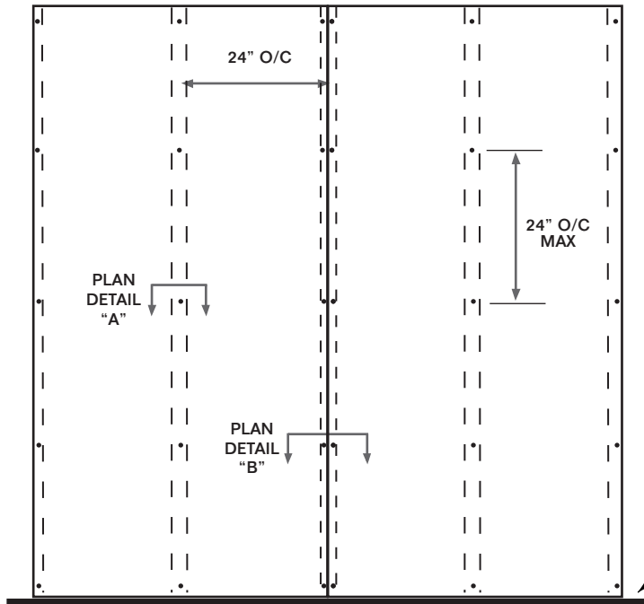
ThermaClad R-12 Panels on Concrete Wall
