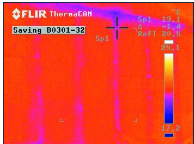
Figure 1a: Thermal photography of stud and batt wall This thermal photograph of a stud wall reveals multiple points where heat can escape – primarily along studs themselves.
