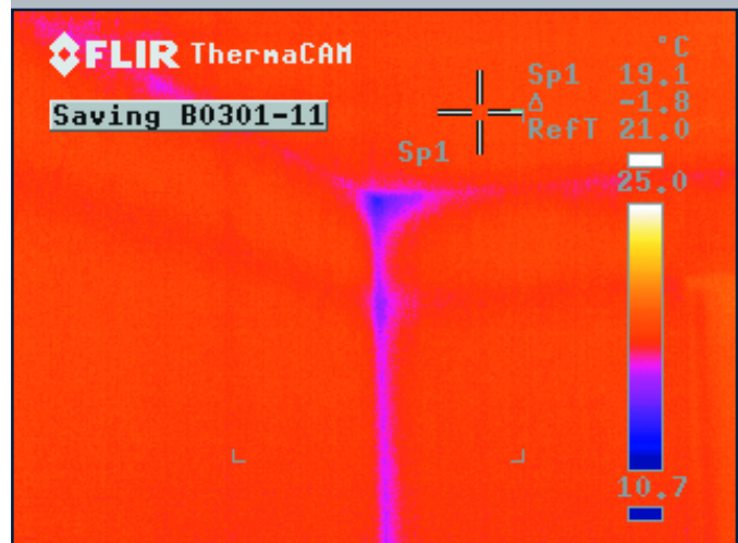
Figure 1b: Thermal photography of SIP wall The SIP wall allows for minimal heat loss along the wall surface. The only heat loss evidenced here occurs in the corner area.
