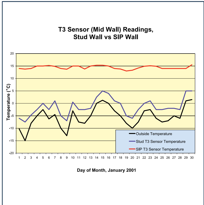
Figure 3: Thermal performance of stud and SIP wall systems
